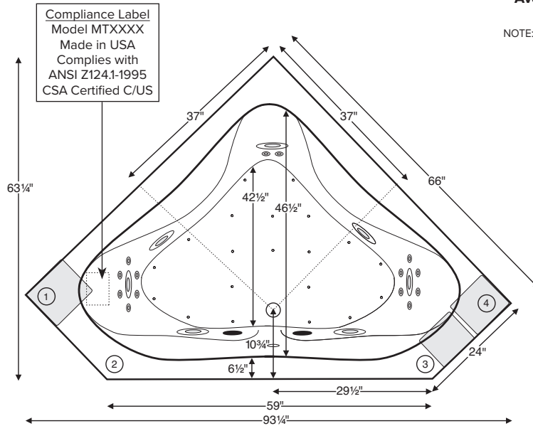
Numbered areas on tub deck represent possible locations to install cleaning systems, faucets and other fixtures.
