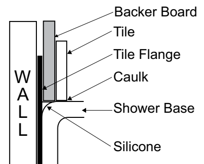
ABS tile flange installed on 3 sides of shower base. Also available on 1 or 2 sides, depending on installation application.
